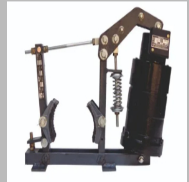
MDT 200-18 Mill Duty Thruster Brakes
