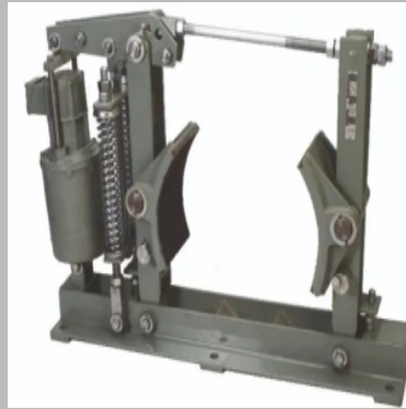
MDT 500-46 Mill Duty Thruster Brakes
