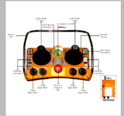
F24-60 Multi Joystick Radio Remote Control System
