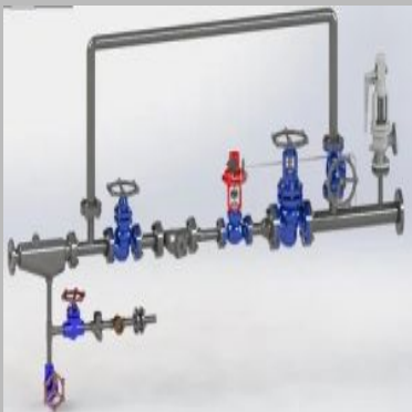
Pressure Reducing Station
