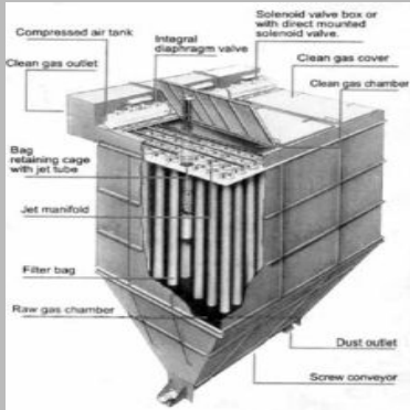
Pulse Jet Bag Filter
