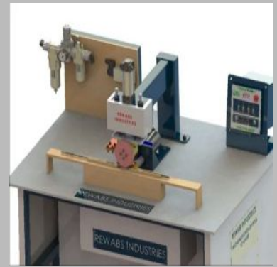
Pneumatic Spot Welding Machine Table Type
