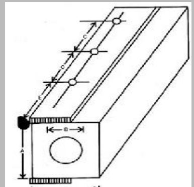
RANELAST Hollow Square Fender
