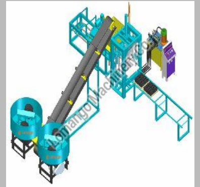
Fully Automatic High Vibration Low Pressure Machine
