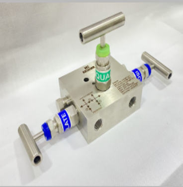
3 Way R Type Manifold Valve
