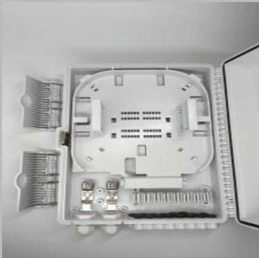
16 Port FTTH Standard Design Optical Terminal Box
