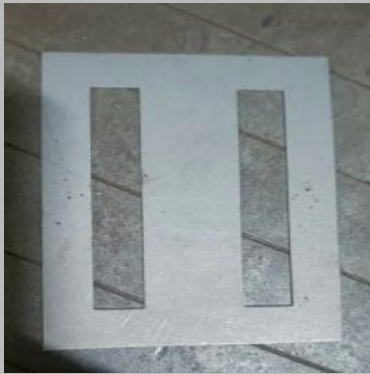
0.27 mm Transformer Lamination
