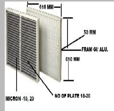
secondary filter
