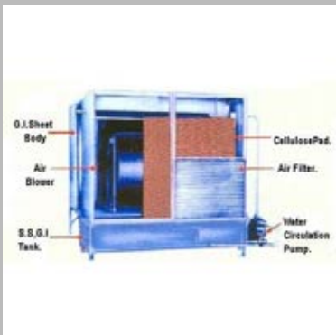
industrial cooler
