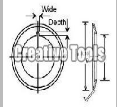
Top Cutter
