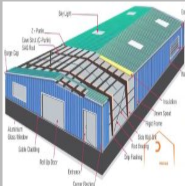
Prefabricated Structure Installation Services
