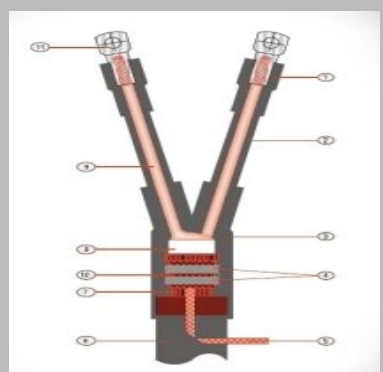
Cable Terminations
