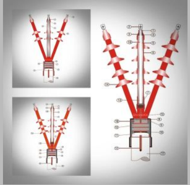
Heat Shrinkable Outdoor Terminations Kit
