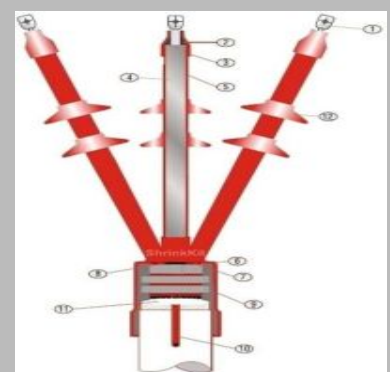
Cable Termination
