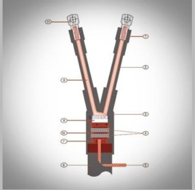
Heat Shrinkable Low Voltage Terminations Kit
