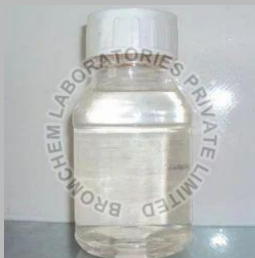
Isovaleryl Chloride
