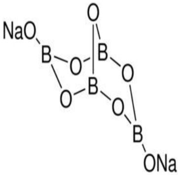
Sodium Tetraborate
